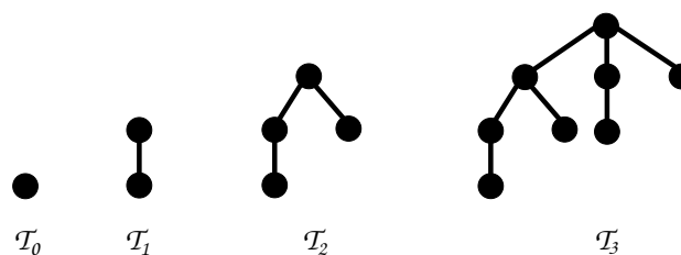
Figure 2: The trees \mathcal{T}_0, \dots, \mathcal{T}_3 .
