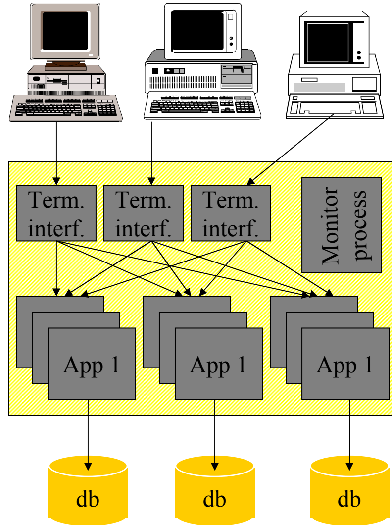
Multiprocessor structure
