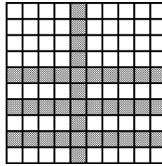
Figure 19.29: An example how to choose a quorum in the f -masking Grid with f = 2 , i.e., 2 + 1 = 3 rows. The load is in \Theta(f/\sqrt{n}) when the access strategy is chosen to be uniform. Two quorums overlap by their columns intersecting each other's rows, i.e., they overlap in at least 2f + 2 nodes.
