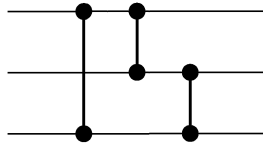
Figure 3: A network that does not sort correctly when fed backwards.
